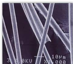
Alumina Fiber (SEM picture)
